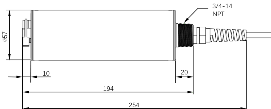
Figure 1 LT-63X Series Dimensions (mm)
