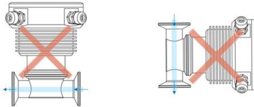
Figure 5. Incorrect Installations
