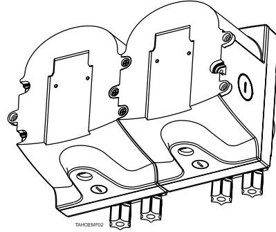
Figure 3. Rear view of two Tahoe units, interlocked with #6 x 1/2" (12mm) self-tapping screws
